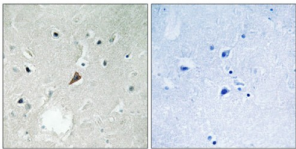
Immunohistochemistry analysis of paraffin-embedded human brain tissue using PYK2 (Phospho-Tyr579) antibody.
