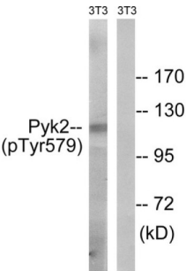
Western blot analysis of extracts from 3T3 cells, using PYK2 (Phospho-Tyr579) antibody.
