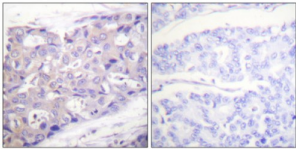
Immunohistochemistry analysis of paraffin-embedded human breast carcinoma tissue using Akt (epitope around residue 326) antibody.
