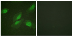
Immunofluorescence analysis of HeLa cells, using Akt (epitope around residue 326) antibody.
