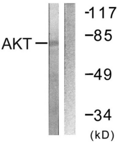
Western blot analysis of extracts from NIH/3T3 cells, treated with Insulin (0.01U/ml, 15mins), using Akt (epitope around residue 326) antibody.
