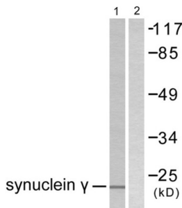
Western blot analysis of extracts from HT29 cells, using Synuclein gamma Antibody (abx013200).
