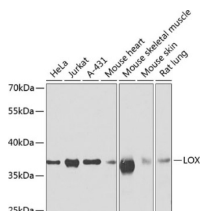
Western blot analysis of extracts of various cell lines using LOX Antibody (1/50 dilution).
