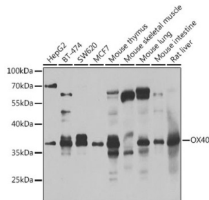
Western blot analysis of extracts of various cell lines using CD134/OX40 Antibody (1/1000 dilution).
