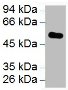
WB analysis of purified alliinase (1/5000 dilution).
