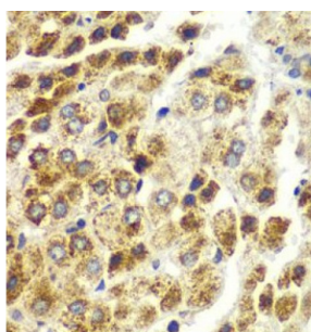
IHC-P analysis of human liver cancer tissue, using SND1 Antibody (1/100 dilution).
