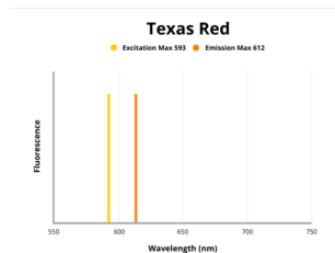
Fluorescence emission spectra of Texas Red.
