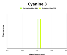
Fluorescence emission spectra of Cyanine 3.
