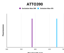
Fluorescence emission spectra of ATTO 390.
