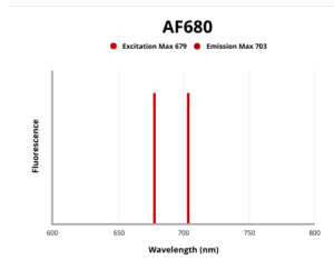
Fluorescence emission spectra of AF680.
