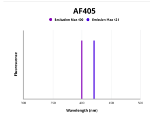
Fluorescence emission spectra of AF405.
