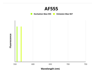
Fluorescence emission spectra of AF555.
