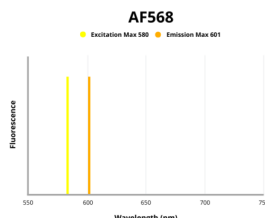
Fluorescence emission spectra of AF568.
