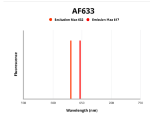
Fluorescence emission spectra of AF633.
