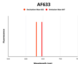
Fluorescence emission spectra of AF633.
