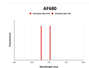
Fluorescence emission spectra of AF680.
