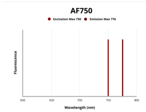
Fluorescence emission spectra of AF750.
