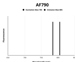
Fluorescence emission spectra of AF790.
