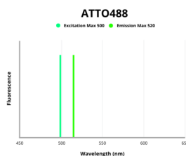
Fluorescence emission spectra of ATTO 488.
