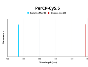
Fluorescence emission spectra of PerCP/Cyanine 5.5.
