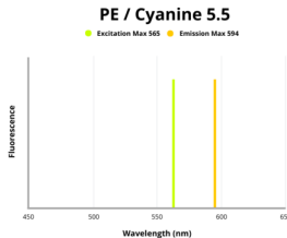
Fluorescence emission spectra of PE/Cyanine 5.5.
