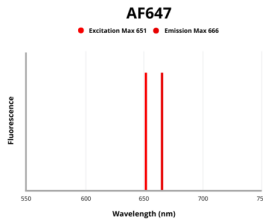
Fluorescence emission spectra of AF647.
