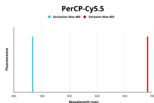
Fluorescence emission spectra of PerCP/Cyanine 5.5.
