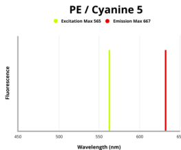
Fluorescence emission spectra of PE/Cyanine 5.
