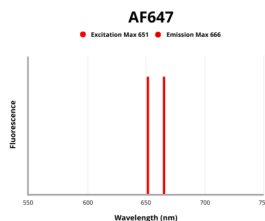
Fluorescence emission spectra of AF647.
