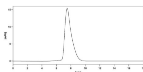
SEC-HPLC analysis of Trontinemab.
