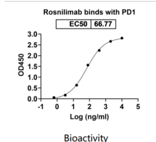
Bioactivity of Rosnilimab
