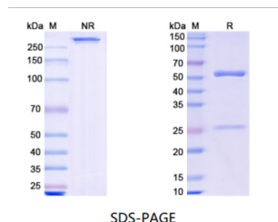
SDS-PAGE analysis of Rosnilimab
