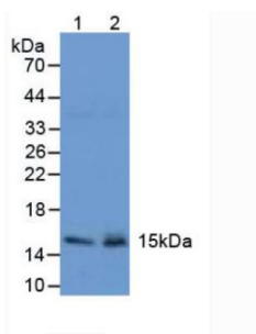
Western blot analysis of (1) Mouse Stomach Tissue and (2) Mouse Pancreas Tissue.
