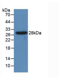
Western blot analysis of recombinant Human CYP1A1.
