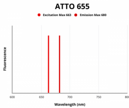
Fluorescence emission spectra of ATTO 655.
