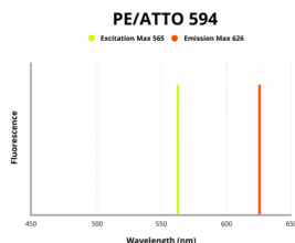
Fluorescence emission spectra of PE/ATTO 594.
